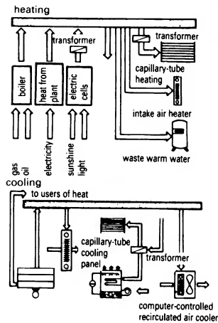
② Air conditioning technology, heating and cooling
